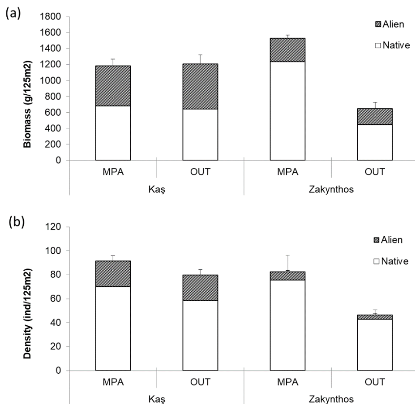
Fig. 1: Composition of native and alien fishes in and out of the Kaş and Zakynthos MPAs in terms of (a) biomass (g/125 m 2 ) and (b) density (individuals/125 m 2 ). The white part of the bar corresponds to native fish and the striped part to aliens.
