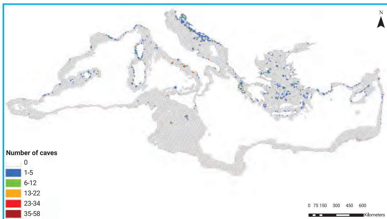
Fig. 2.1. Distribution of marine caves in the Mediterranean Sea. Different colours indicate the number of caves recorded in cells of 10 x 10 km (from Giakoumi et al. , 2013).
