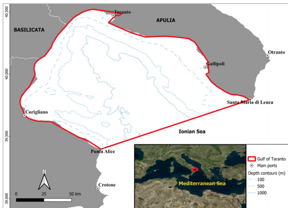
Figure 1. Map of Gulf of Taranto (red polygon). The most important ports are reported.
