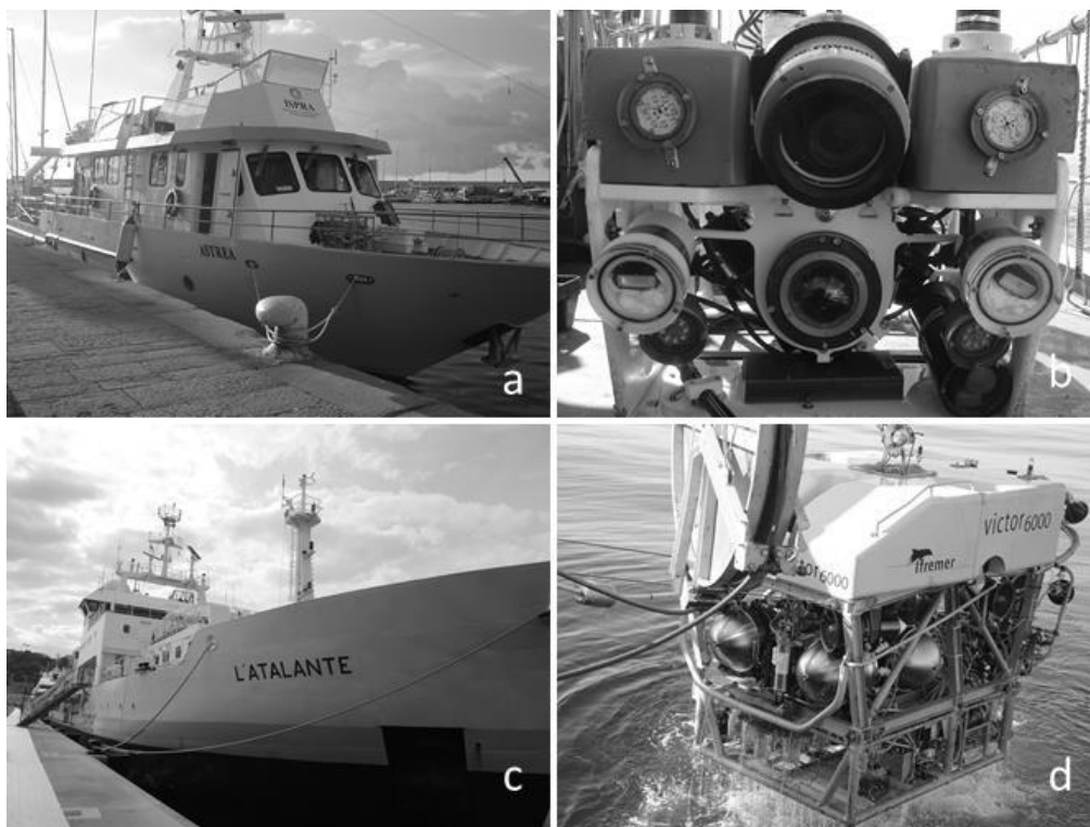
Fig. 2: a) Oceanographic vessel “R/V Astrea” used during the 2015 campaign; b) ROV “Pollux III” used during the 2015 campaign; c) Oceanographic vessel “N/O Atalante” used during the 2018 campaign; d) ROV Victor 6000 used during the 2018 campaign (Photos by B. Daniel/AFB).
