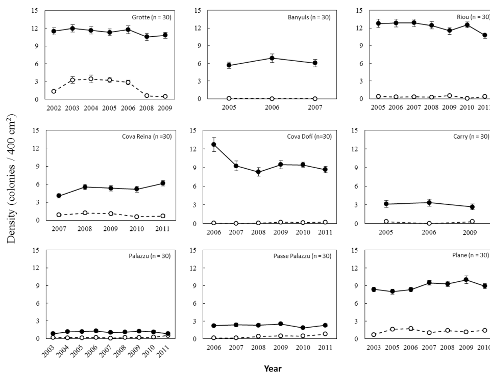
Fig. 1: Long-term population trends at nine red coral populations in the NW Mediterranean. Black dots indicate adult and white dots recruit densities
